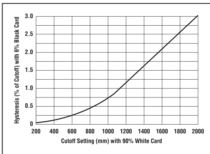
Figure 12. Q60 hysteresis
